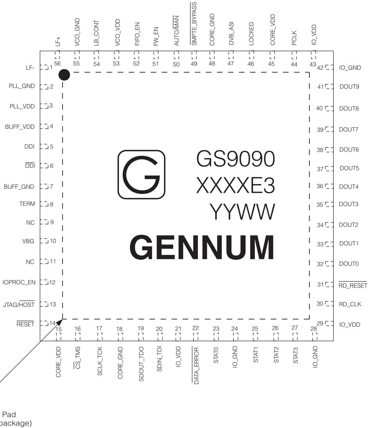
Figure 1-1: Pin Assignment
